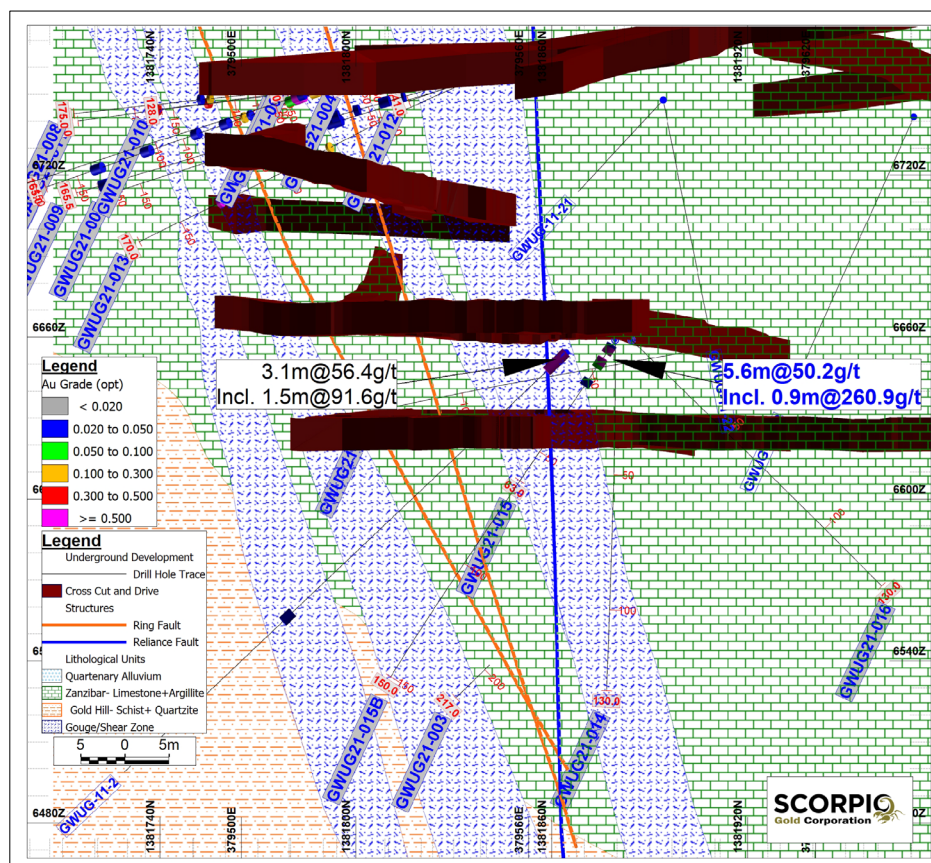
Figure 2: Cross-section within 10m projection volume showing significant intercepts for GWUG21-015
