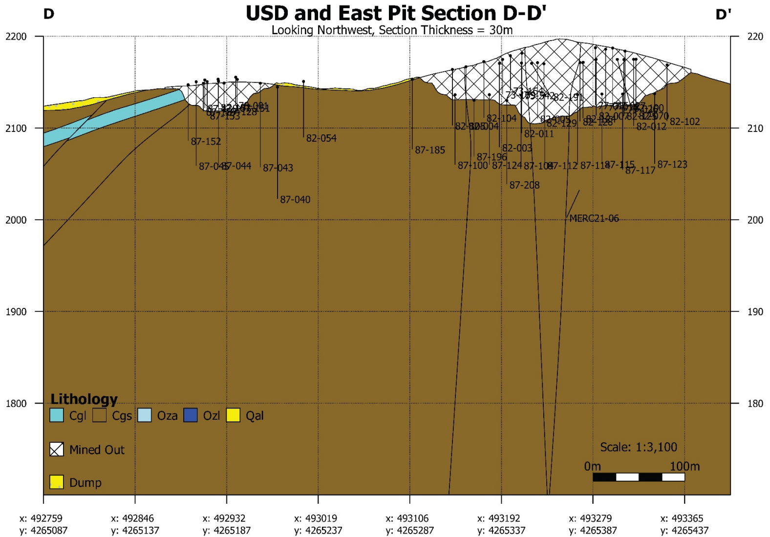
Figure 10-5: USD and East Pit Section D-D' (Loury, 2025)
