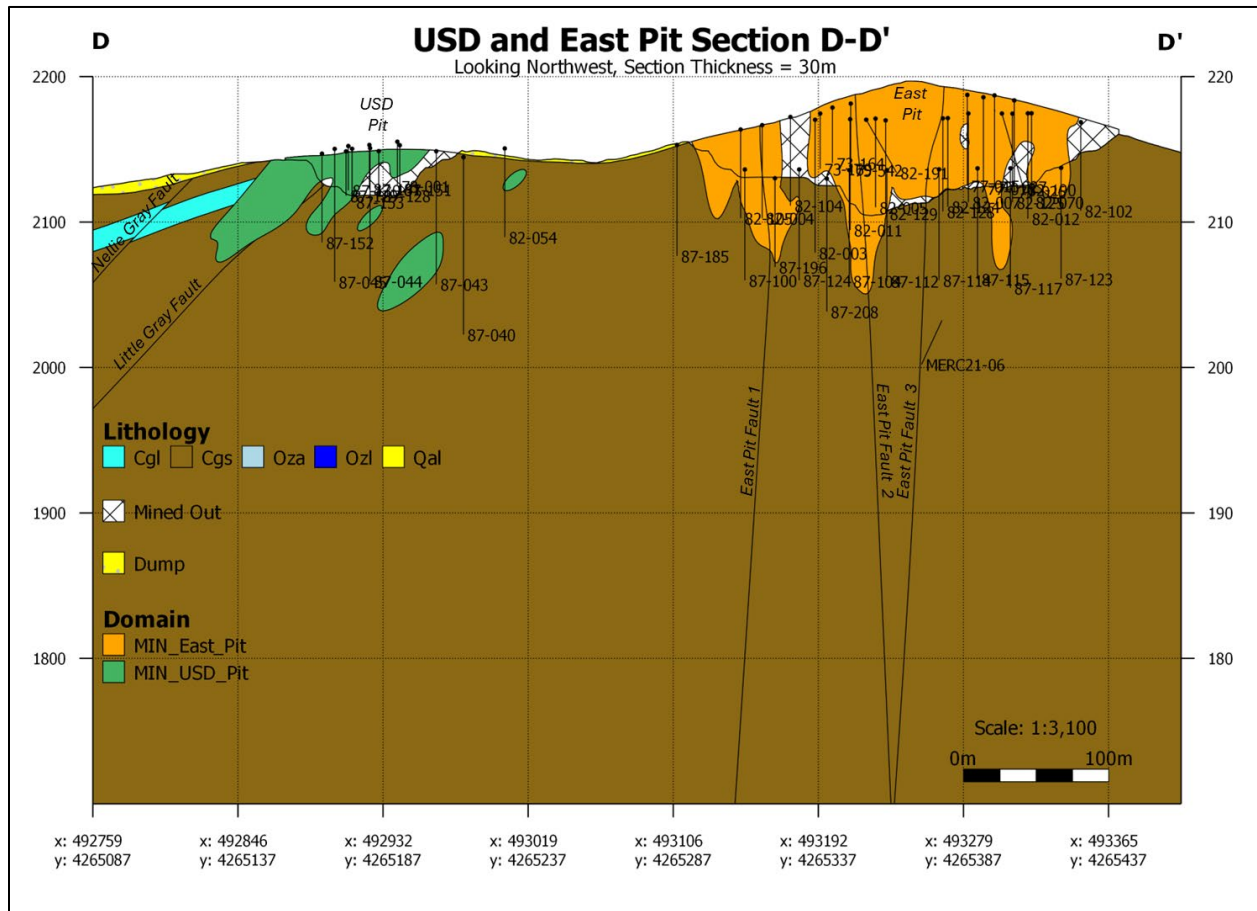
Figure 14-10: Section D-D' showing the MIN_East_Pit and MIN_USD_Pit estimation domains (Loury, 2025)
