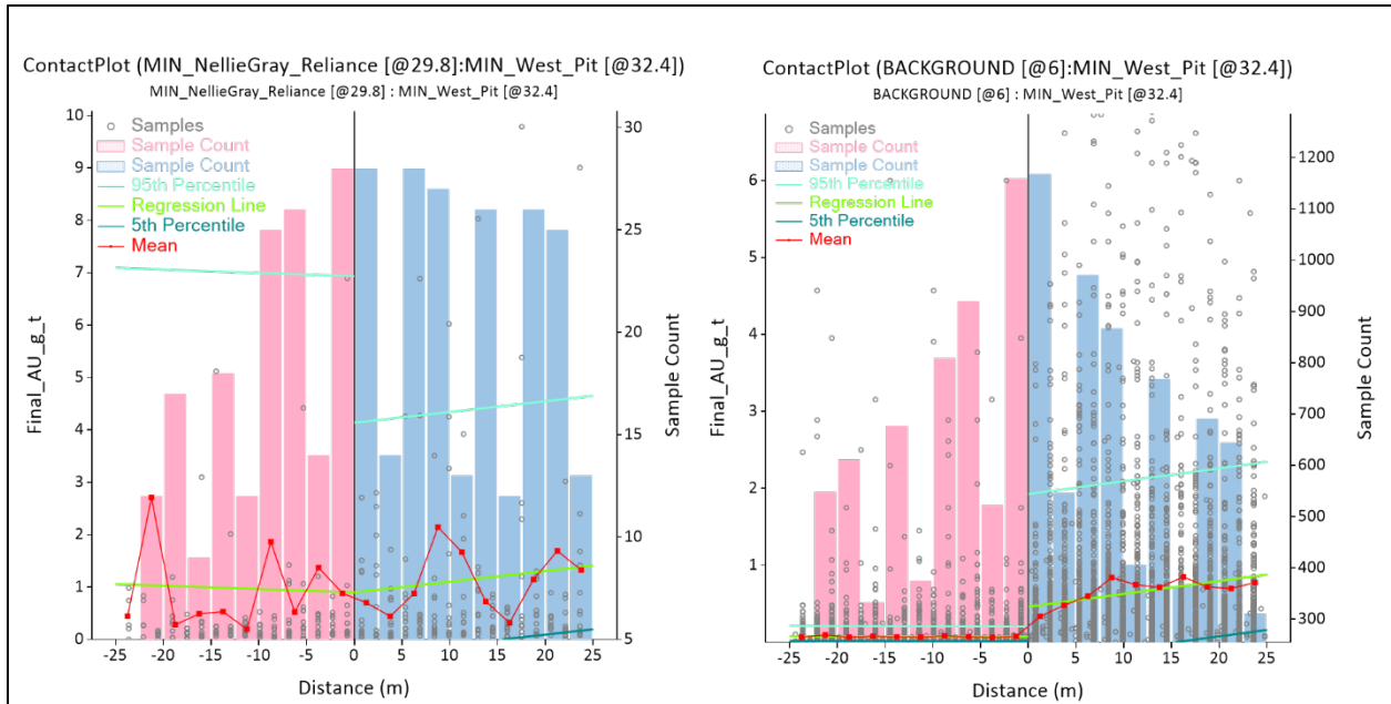
Figure 14-12: Contact plot examples from the MIN_West_Pit domain (Loury, 2025)
