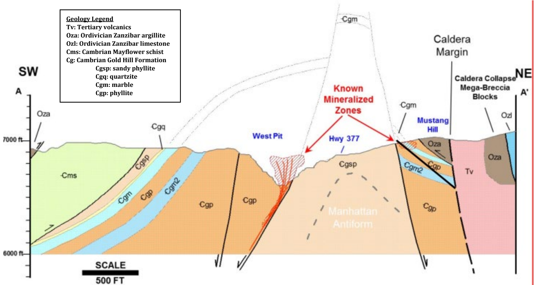
Figure 7-3: Generalized Cross Section
