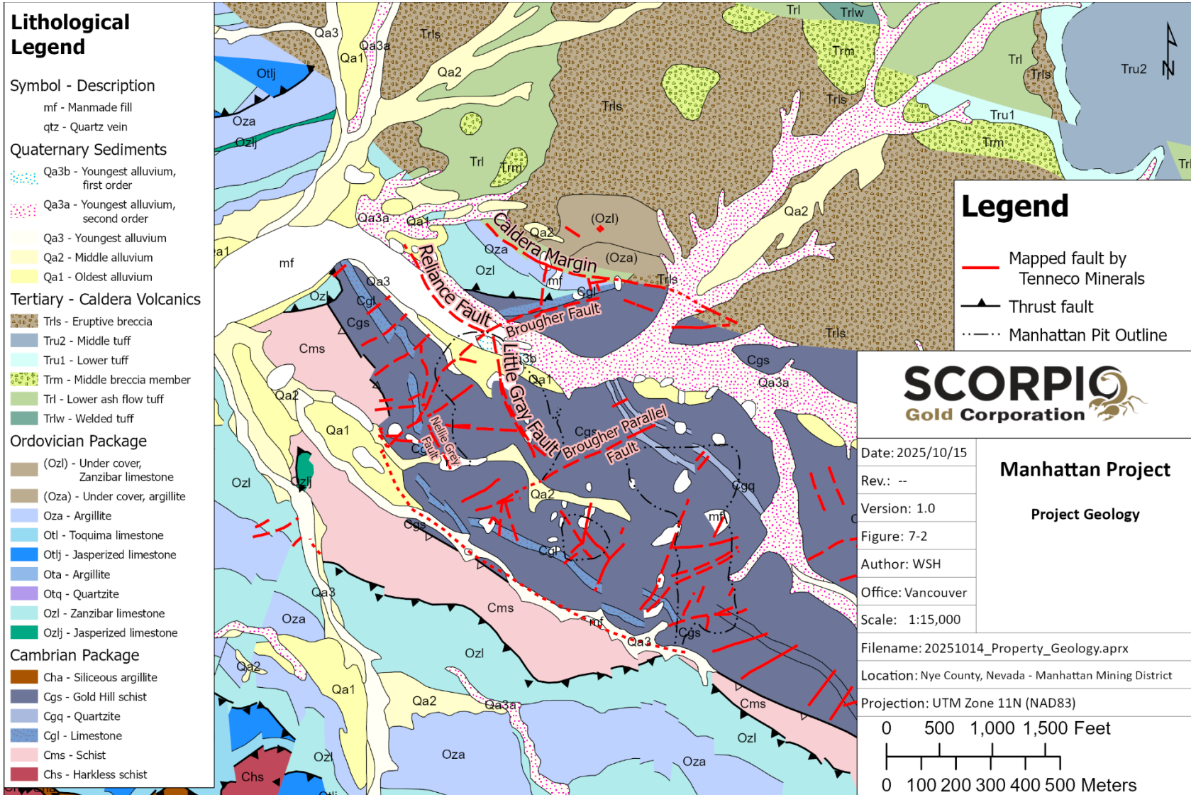
Figure 7-2: Property Geology
